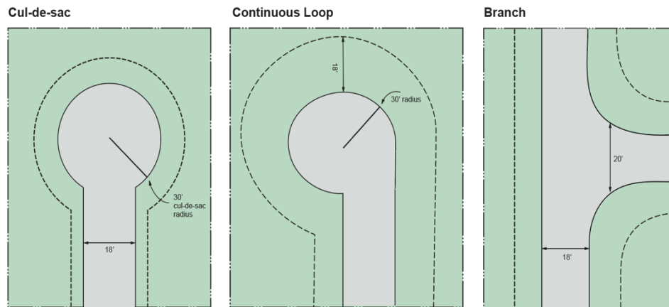
Figure 10-3: Turnarounds
